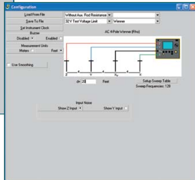
Soil resistivity test setup screen — operator can select either the Wenner or Schlumberger test method, select test voltage and frequency and program the spacing between electrodes in either feet or meters.
