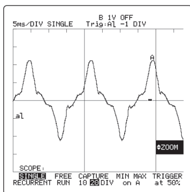
Figure 4. Phase current
