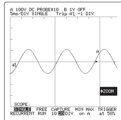
Figure 1. Near sine wave
