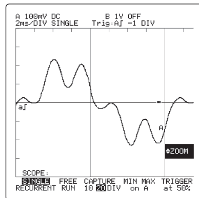
Figure 3B. Three-phase, non-linear load current waveform
