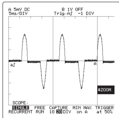
Figure 3A. Single-phase, non-linear load current waveform
