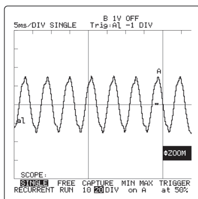
Figure 5. Neutral current
